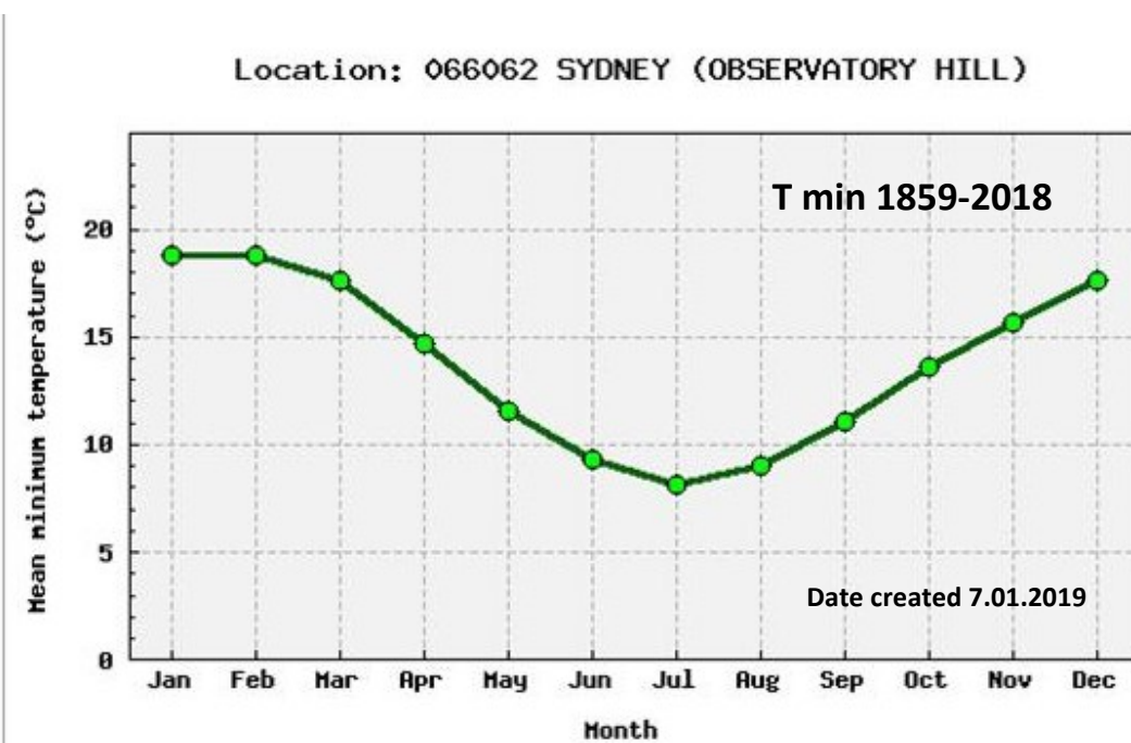
Figure 10: T min data from Sydney Observatory for the period 1859 –2018, in degrees C (from BOM)
